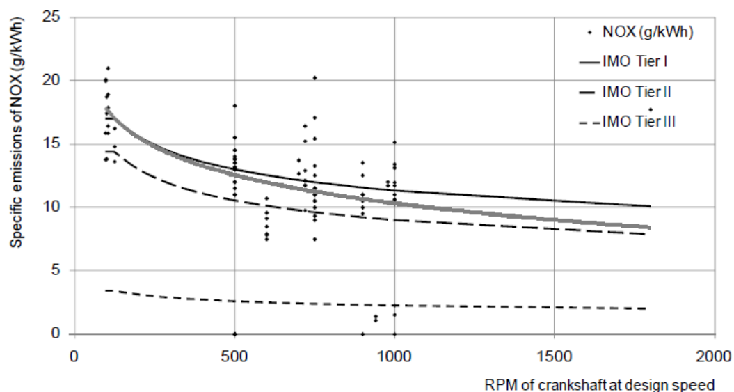
Figure.2.: The specific emissions measurements from ships and test bed measurements in Wärtsilä's facility (Whall et al. 2002; Agrawal et al. 2008; Winnes and Fridell 2009; Winnes and Fridell 2010).
