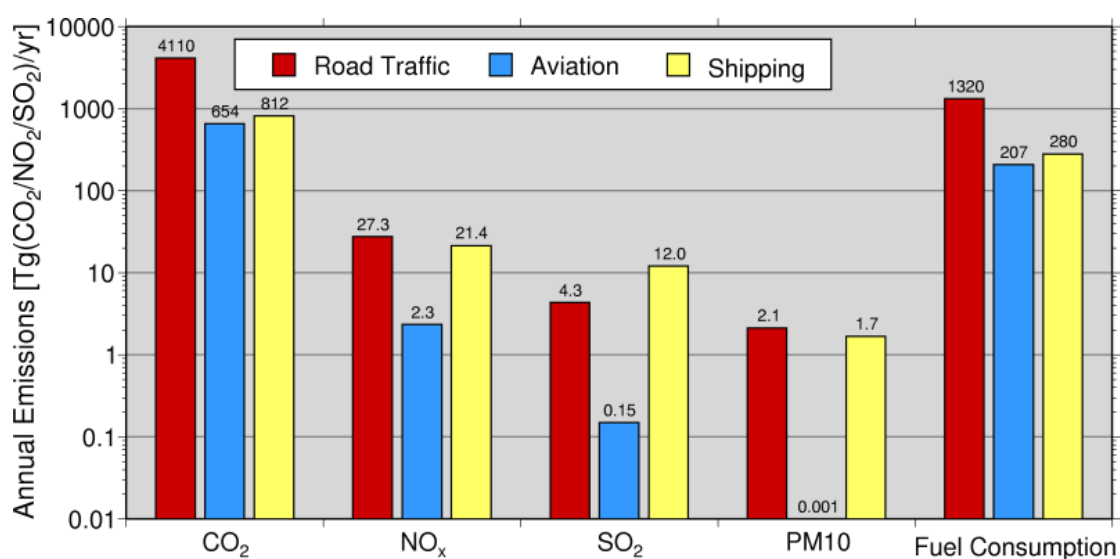
Figure.6.: [Transport-related annual emissions of CO 2 , NO x , SO 2 and PM 10 and the fuel consumption in Tg (1 Tg = 1 \times 10^{12} g = Mt) estimated for the year 2000; Eyring et al. (2005a) ].
